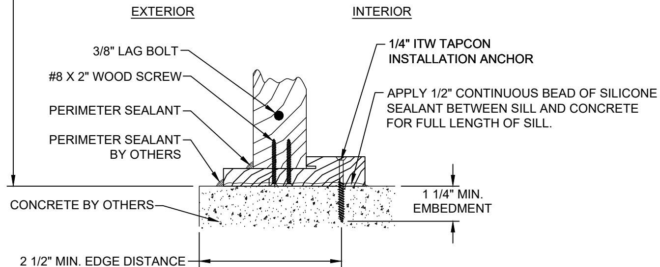
E VERTICAL SECTION GLAZED SIDELITE PANEL AT SILL CONCRETE / MASONRY SUBSTRATE OUTSWING SHOWN / INSWING OPPOSITE (SEE SHEET 3 SECTIONS 1, 2 & 3 FOR APPROPRIATE SIDELITE PANELS)
