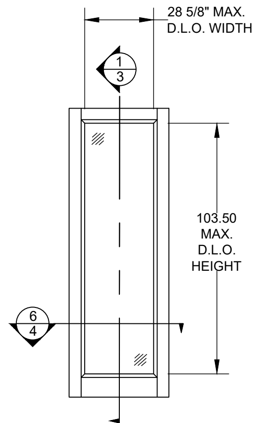
FULL LITE (DOOR & SIDELITE PANELS)
