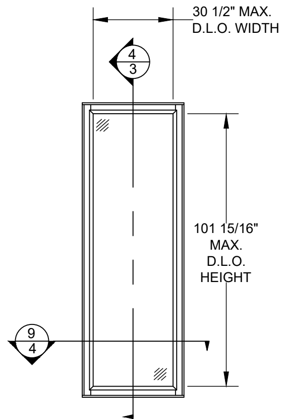
FULL LITE (DOOR & SIDELITE PANELS)
