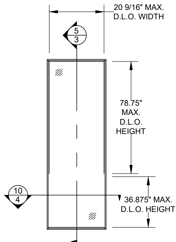
DIRECT SET PANEL (SIDELITE PANEL)
