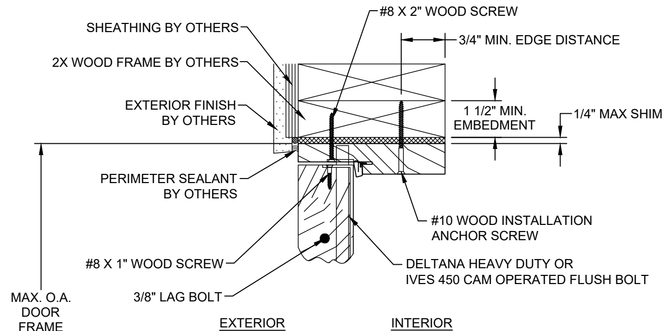
D VERTICAL SECTION GLAZED DOOR PANEL AT HEAD WOOD FRAME SUBSTRATE OUTSWING SHOWN / INSWING OPPOSITE (SEE SHEET 3 SECTIONS 1, 2 & 3 FOR APPROPRIATE DOOR PANELS)
