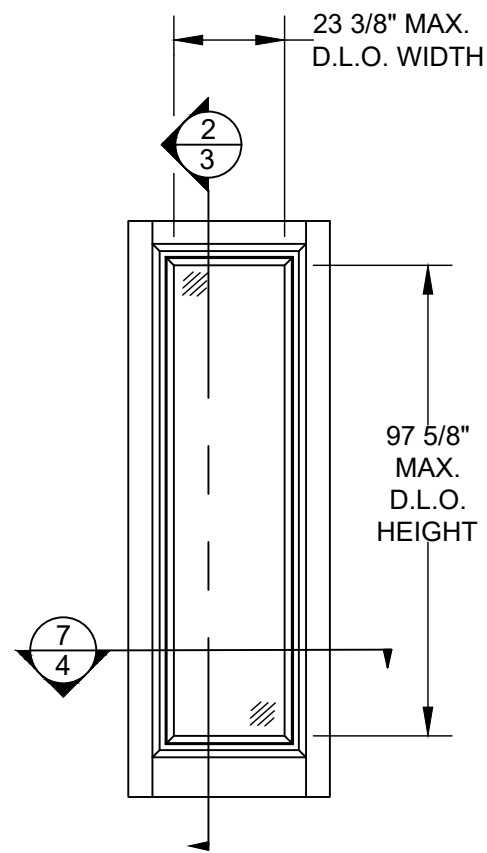
FULL LITE PANEL INSERT (DOOR & SIDELITE PANELS)
