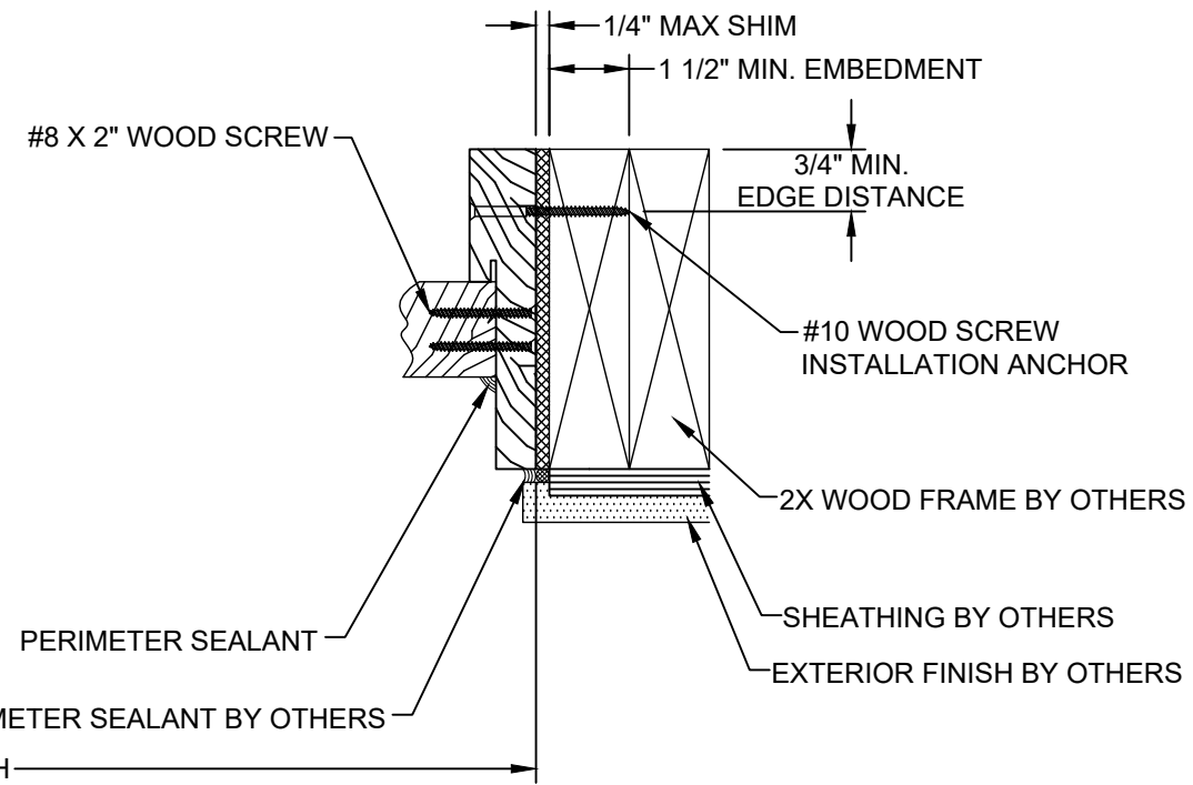
HORIZONTAL SECTION GLAZED SASH SET SIDELITE PANEL AT JAMB WOOD FRAME SUBSTRATE OUTSWING SHOWN / INSWING OPPOSITE (SEE SHEET 4 SECTION 9 & 12 FOR APPROPRIATE SIDELITE PANELS)
