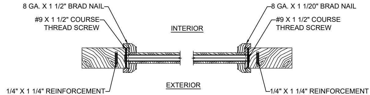
8 4 HORIZONTAL CROSS SECTION WOOD PANEL UNDER 3/4 LITE GLAZING DOOR & SIDELITE PANELS
