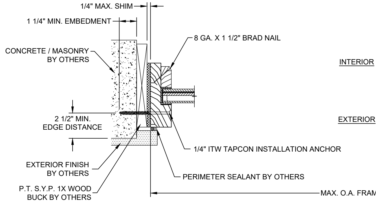
HORIZONTAL SECTION GLAZED DIRECT SET SIDELITE PANEL AT JAMB CONCRETE / MASONRY SUBSTRATE OUTSWING SHOWN / INSWING OPPOSITE (SEE SHEET 4 SECTION 10 FOR APPROPRIATE SIDELITE PANEL)
