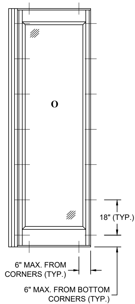
ANCHOR LAYOUT OPTIONAL SASH SET SIDELITE GLAZED OR OPAQUE (GLAZED SHOWN) EXTERIOR VIEW
