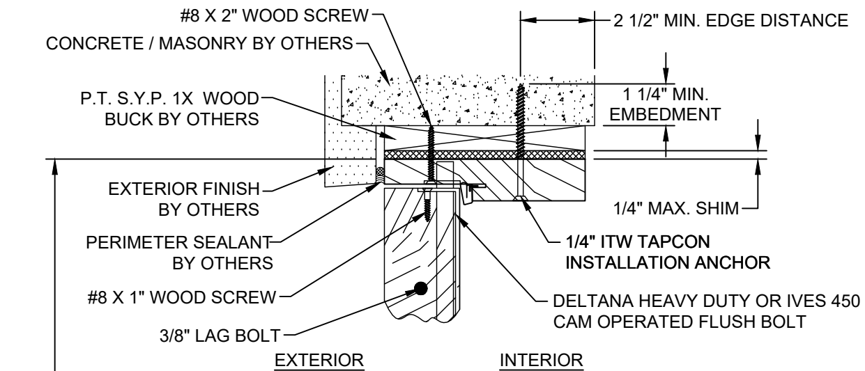
C VERTICAL SECTION GLAZED DOOR PANEL AT HEAD CONCRETE / MASONRY SUBSTRATE OUTSWING SHOWN / INSWING OPPOSITE (SEE SHEET 3 SECTIONS 1, 2 & 3 FOR APPROPRIATE DOOR PANELS)
