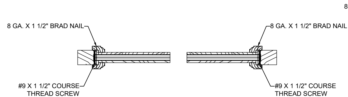
12 4 HORIZONTAL CROSS SECTION OPAQUE SASH SET SIDELITE PANEL
