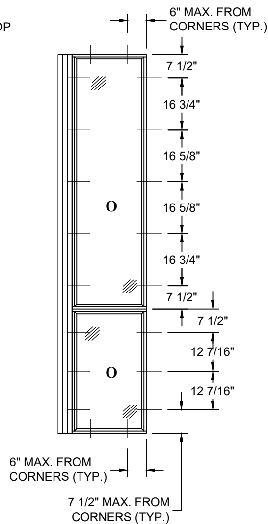
ANCHOR LAYOUT OPTIONAL DIRECT SET SIDELITE EXTERIOR VIEW
