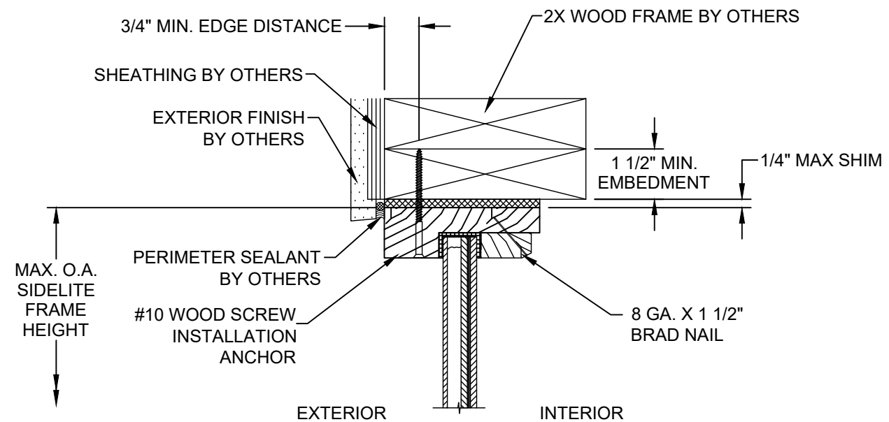
J VERTICAL SECTION GLAZED DIRECT SET SIDELITE PANEL AT HEAD WOOD FRAME SUBSTRATE OUTSWING SHOWN / INSWING OPPOSITE (SEE SHEET 3 SECTION 5 FOR APPROPRIATE SIDELITE PANEL)
