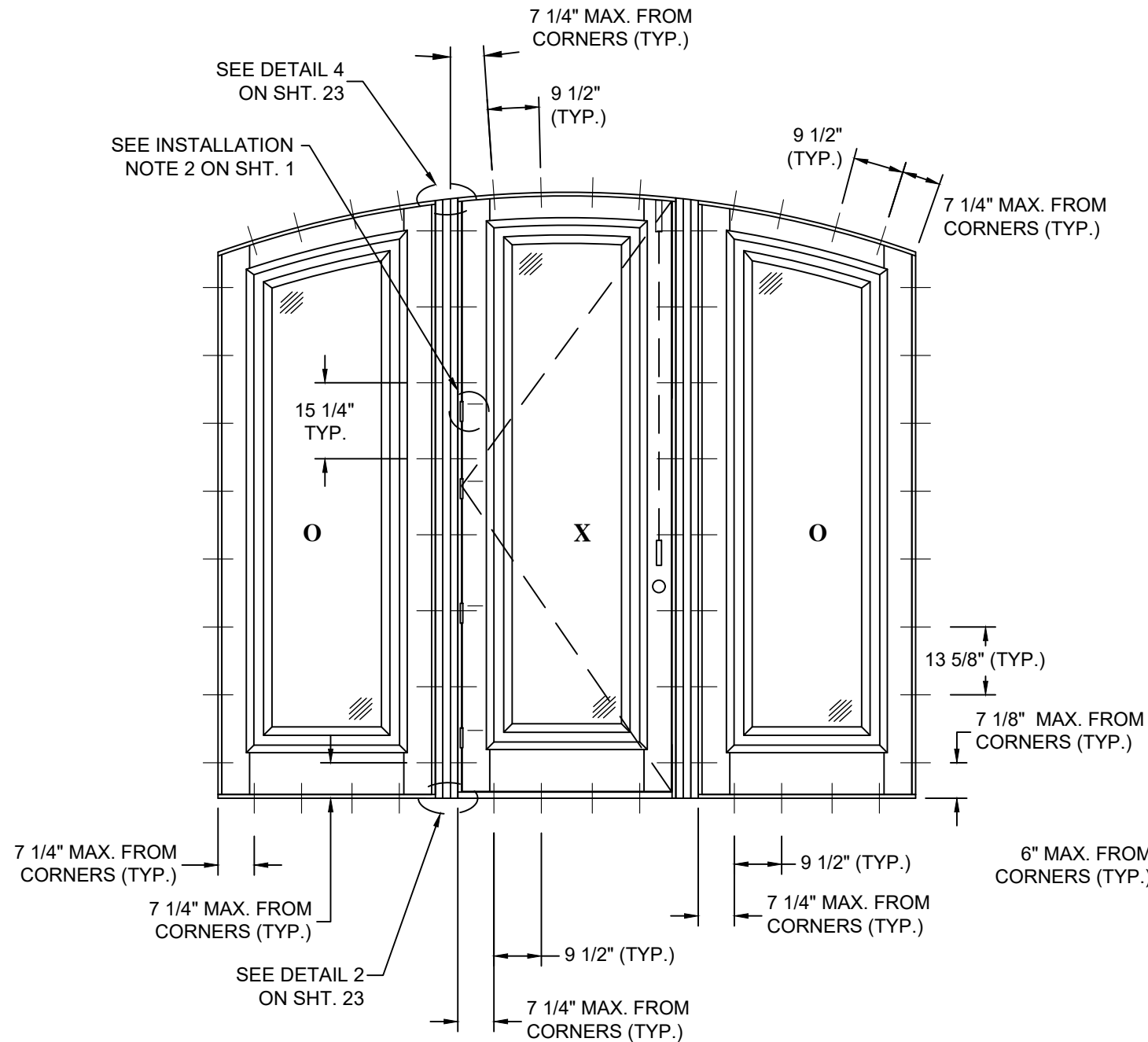
ANCHOR LAYOUT OPTIONAL EYEBROW TOP INSWING / OUTSWING (OXO) EXTERIOR VIEW
