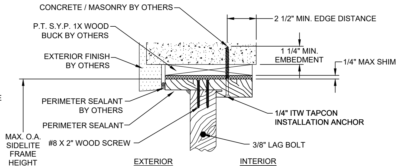
L VERTICAL SECTION GLAZED SASH SET SIDELITE PANEL AT SILL CONCRETE / MASONRY SUBSTRATE OUTSWING SHOWN / INSWING OPPOSITE (SEE SHEET 3 SECTION 4 & 11 FOR APPROPRIATE SIDELITE PANELS)
