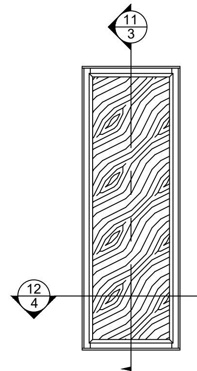
OPAQUE SASH SET PANEL (SIDELITE PANEL)
