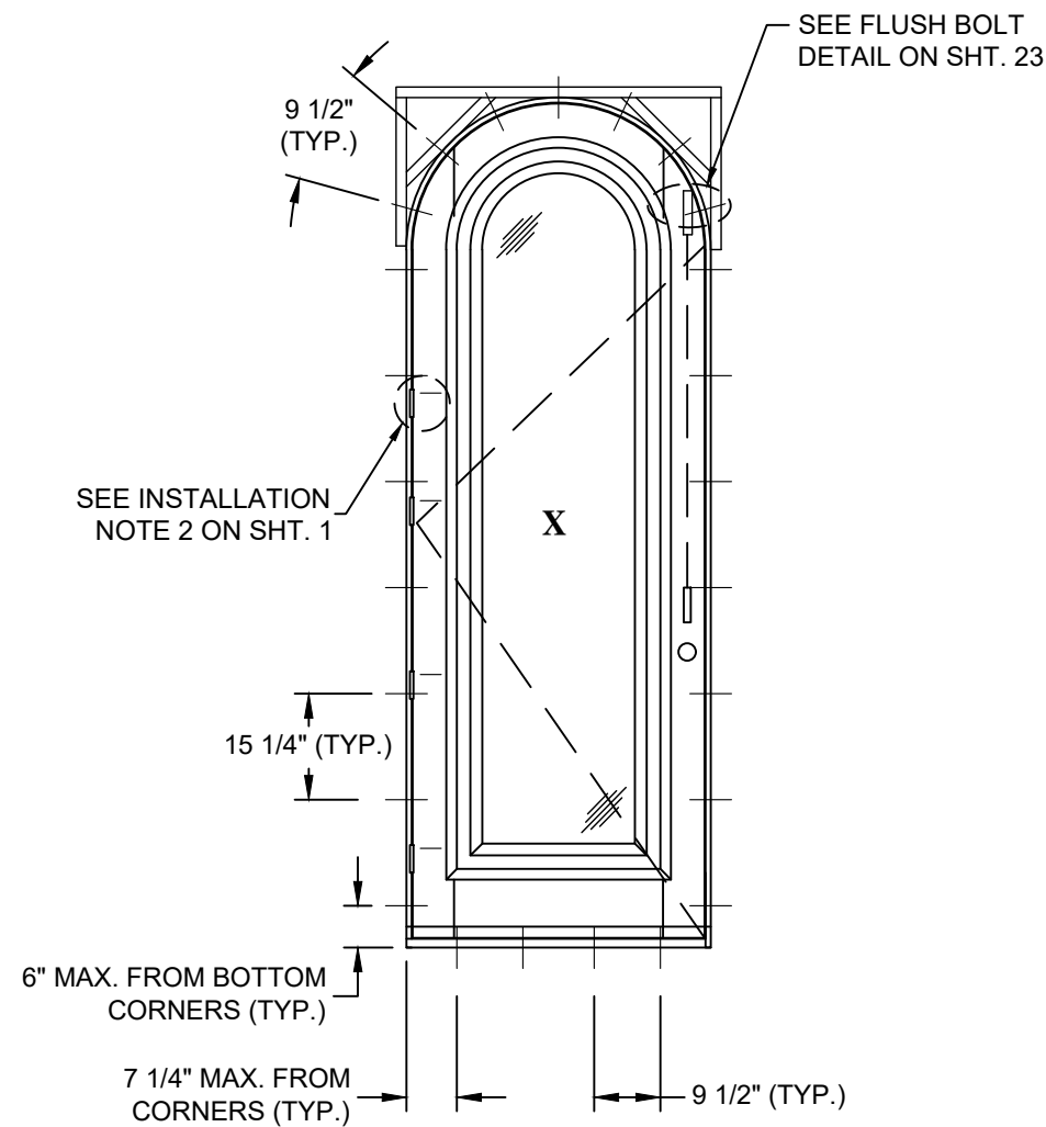
ANCHOR LAYOUT OPTIONAL ROUND TOP INSWING / OUTSWING (X) FULL LITE PANEL INSERT DOOR EXTERIOR VIEW
