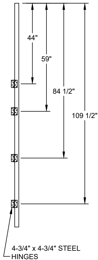
HINGE LOCATIONS
