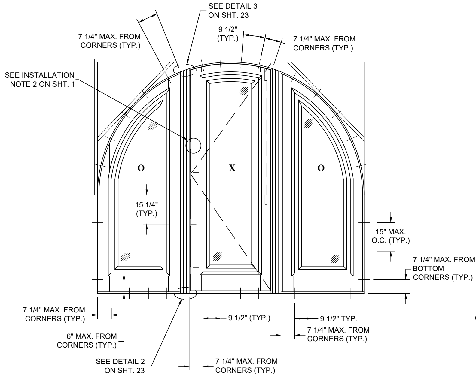
ANCHOR LAYOUT OPTIONAL RADIUS TOP INSWING / OUTSWING (OXO) EXTERIOR VIEW
