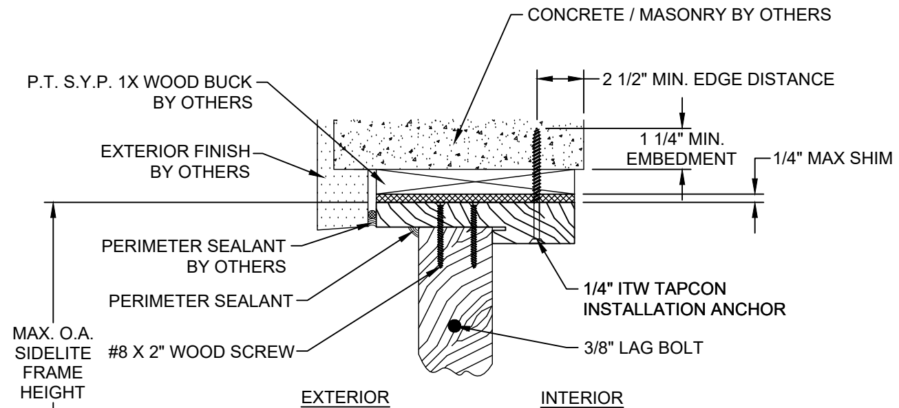
F VERTICAL SECTION GLAZED SIDELITE PANEL AT HEAD CONCRETE / MASONRY SUBSTRATE OUTSWING SHOWN / INSWING OPPOSITE (SEE SHEET 3 SECTIONS 1, 2 & 3 FOR APPROPRIATE SIDELITE PANELS)
