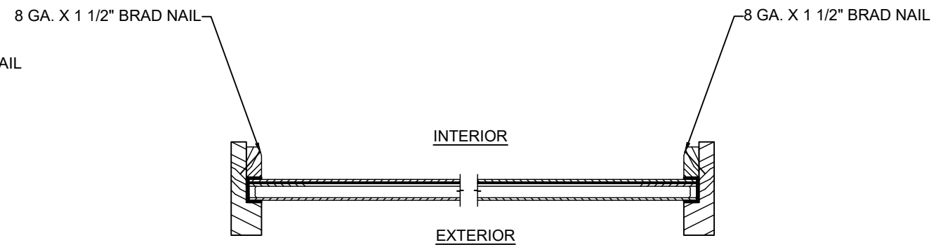
10 4 HORIZONTAL CROSS SECTION DIRECT SET SIDELITE PANEL
