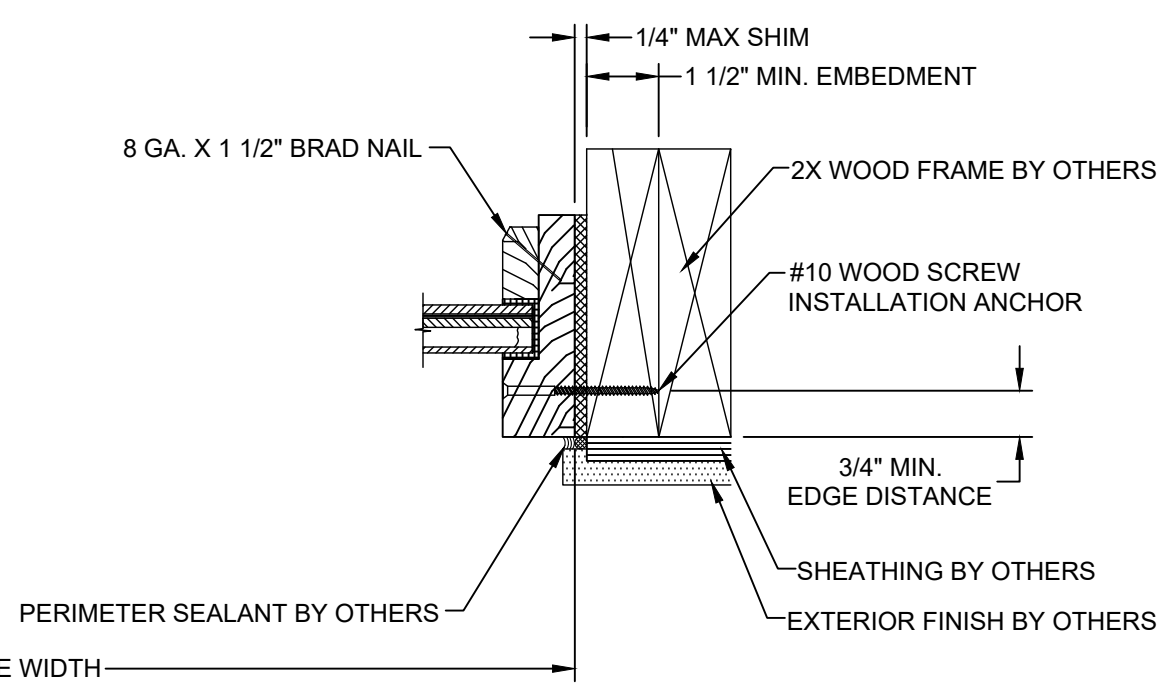
HORIZONTAL SECTION GLAZED DIRECT SET SIDELITE PANEL AT JAMB WOOD FRAME SUBSTRATE OUTSWING SHOWN / INSWING OPPOSITE (SEE SHEET 4 SECTION 10 FOR APPROPRIATE SIDELITE PANEL)
