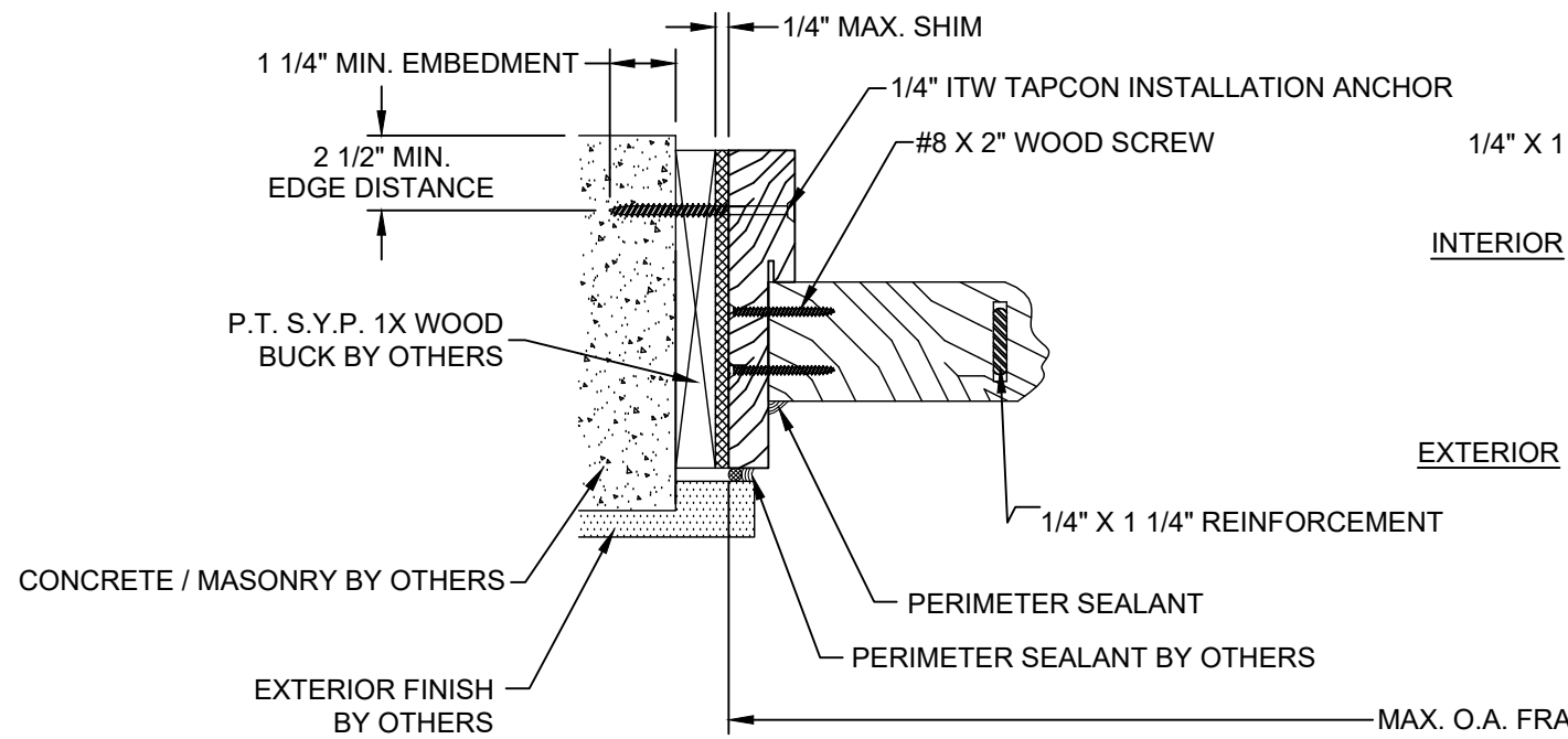
HORIZONTAL SECTION GLAZED SIDELITE PANEL AT JAMB CONCRETE / MASONRY SUBSTRATE OUTSWING SHOWN / INSWING OPPOSITE (SEE SHEET 4 SECTIONS 6, 7 & 8 FOR APPROPRIATE SIDELITE PANELS)
