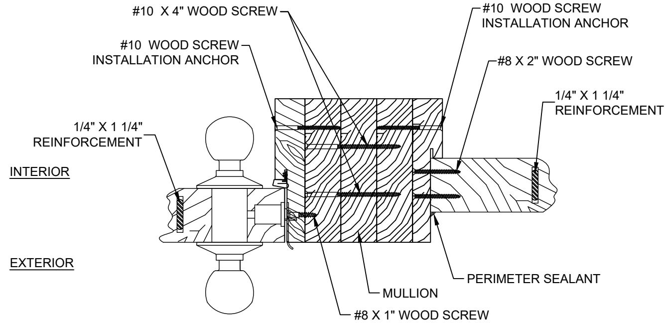
HORIZONTAL SECTION GLAZED DOOR PANEL / GLAZED SIDELITE PANEL AT MULLION OUTSWING SHOWN / INSWING OPPOSITE (SEE SHEET 4 SECTIONS 6, 7 & 8 FOR APPROPRIATE DOOR & SIDELITE PANELS)
