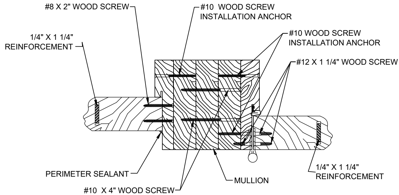
HORIZONTAL SECTION GLAZED SIDELITE PANEL / GLAZED DOOR PANEL AT MULLION OUTSWING SHOWN / INSWING OPPOSITE (SEE SHEET 4 SECTIONS 6, 7 & 8 FOR APPROPRIATE DOOR & SIDELITE PANELS)
