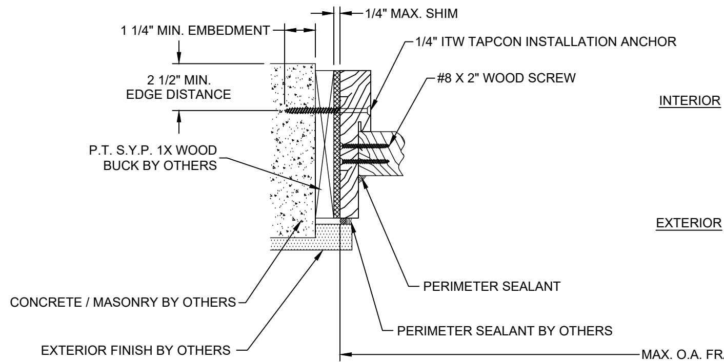
HORIZONTAL SECTION GLAZED SASH SET SIDELITE PANEL AT JAMB CONCRETE / MASONRY SUBSTRATE OUTSWING SHOWN / INSWING OPPOSITE (SEE SHEET 4 SECTION 9 & 12 FOR APPROPRIATE SIDELITE PANELS)
