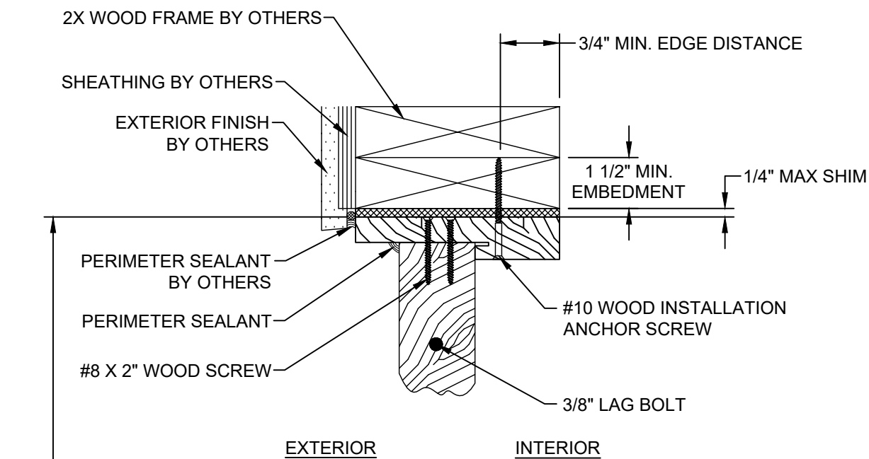
G VERTICAL SECTION GLAZED SIDELITE PANEL AT HEAD WOOD FRAME SUBSTRATE OUTSWING SHOWN / INSWING OPPOSITE (SEE SHEET 3 SECTIONS 1, 2 & 3 FOR APPROPRIATE SIDELITE PANELS)
