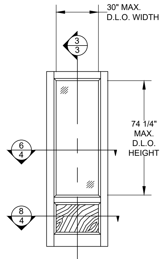
3/4 LITE OVER WOOD PANEL (DOOR & SIDELITE PANELS)
