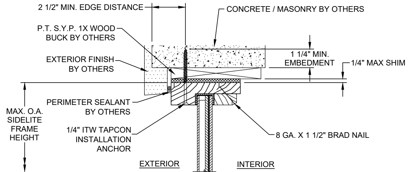
I VERTICAL SECTION GLAZED DIRECT SET SIDELITE AT HEAD CONCRETE / MASONRY SUBSTRATE OUTSWING SHOWN / INSWING OPPOSITE (SEE SHEET 3 SECTION 5 FOR APPROPRIATE SIDELITE PANEL)
