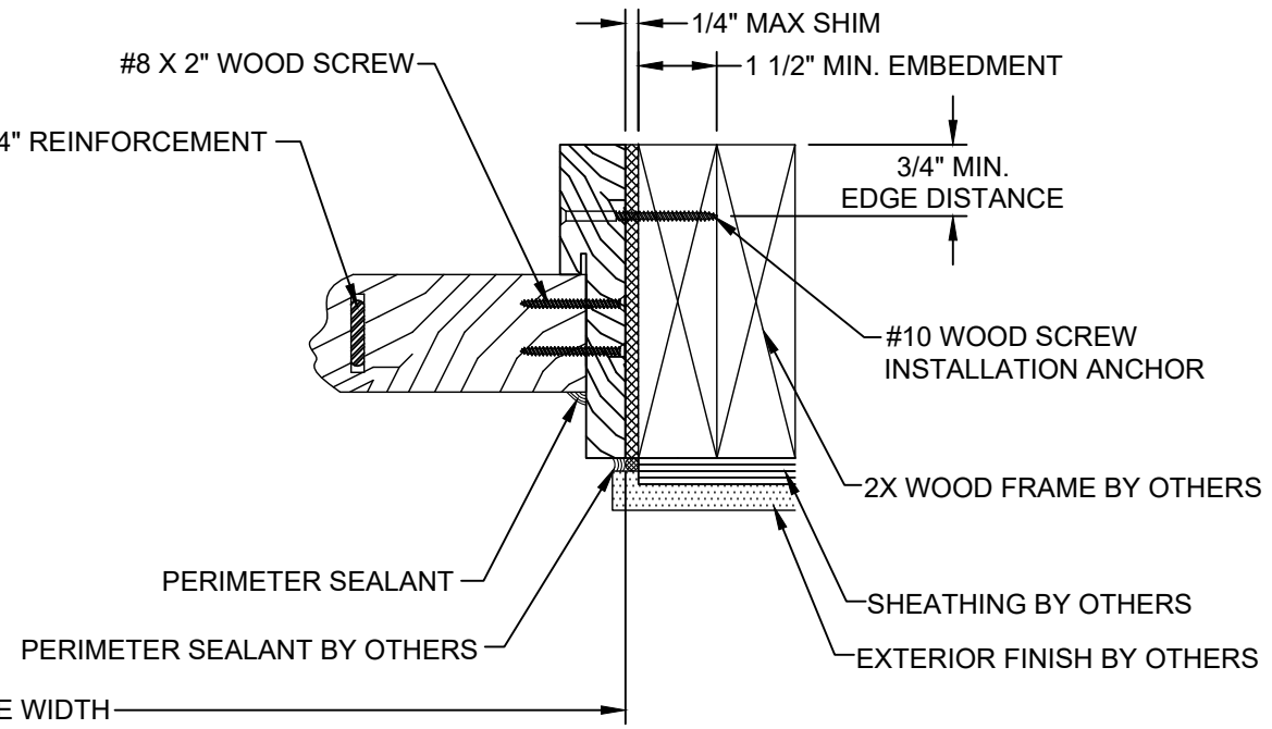
HORIZONTAL SECTION GLAZED SIDELITE PANEL AT JAMB WOOD FRAME SUBSTRATE OUTSWING SHOWN / INSWING OPPOSITE (SEE SHEET 4 SECTIONS 6, 7 & 8 FOR APPROPRIATE SIDELITE PANEL)
