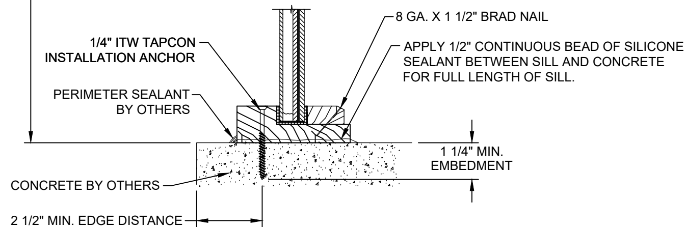
H VERTICAL SECTION GLAZED DIRECT SET SIDELITE PANEL AT SILL CONCRETE / MASONRY SUBSTRATE OUTSWING SHOWN / INSWING OPPOSITE (SEE SHEET 3 SECTION 5 FOR APPROPRIATE SIDELITE PANEL)
