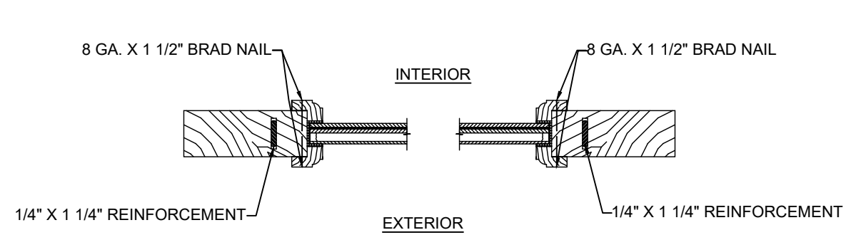
6 4 HORIZONTAL CROSS SECTION FULL LITE DOOR & 3/4 LITE OVER WOOD DOOR PANEL & SIDELITE PANELS
